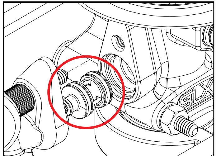
Fig. 10.3: SLX Check Valve at air inlet (correct orientation)
