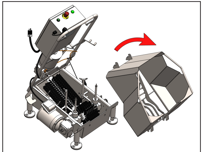
Fig. 8.2: Removing grate
